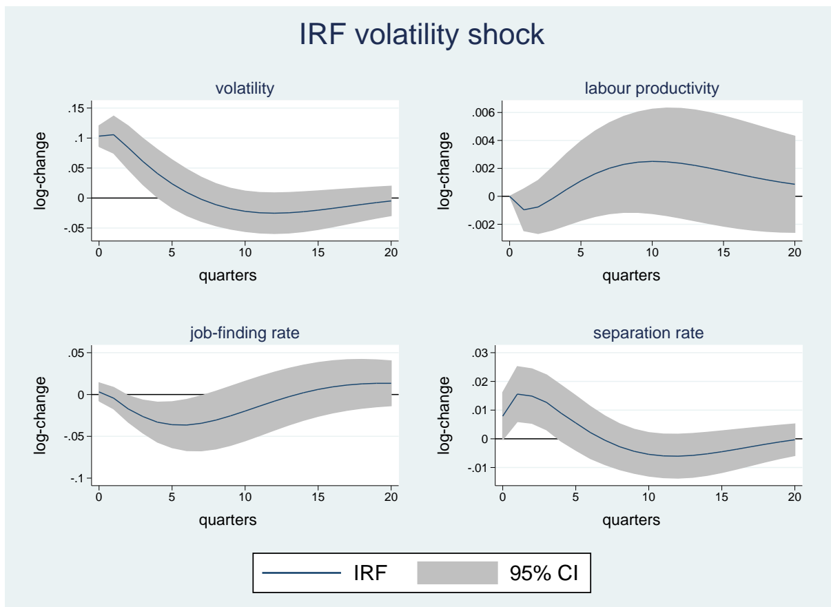
Figure 2: Impulse response functions after a volatility shock in US data.
