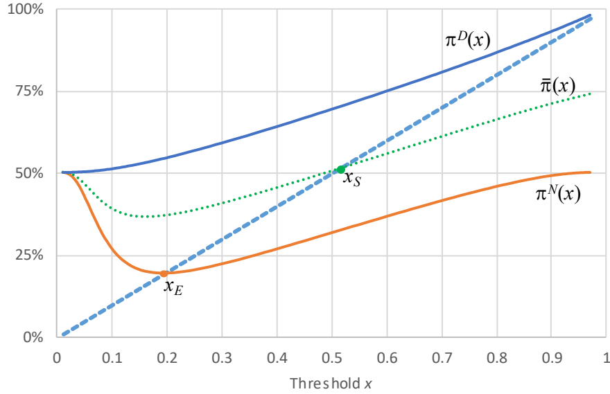
Figure 3: Informationally-Efficient Threshold x_S versus Equilibrium Threshold x_E . (Parameters as in Figure 1.)
